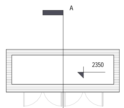
5 Roof Plan 1:100
