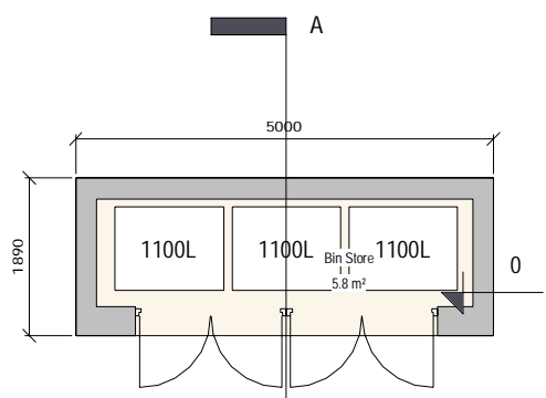
1 Ground Floor Plan 1:100
