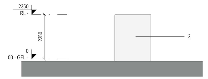
3 Side Elevation A 1:100
