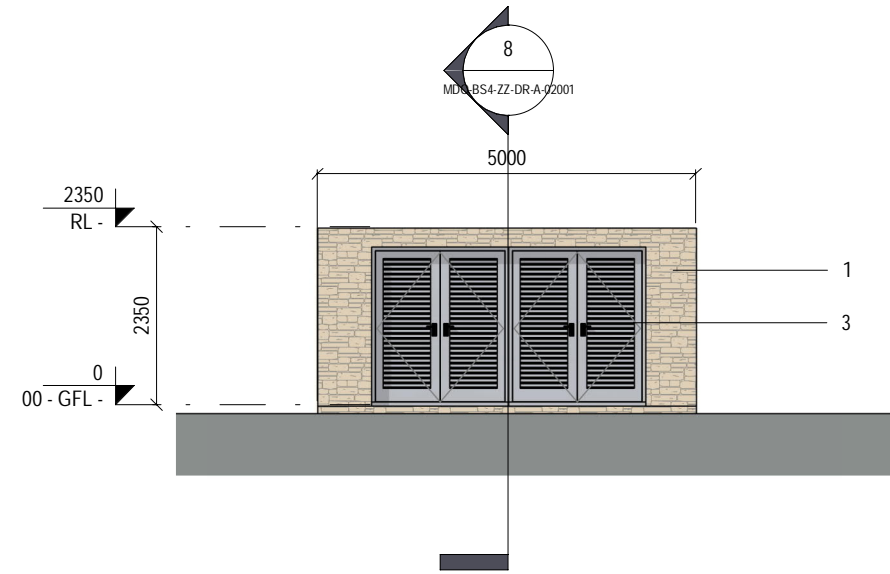
2 Front Elevation 1:100
